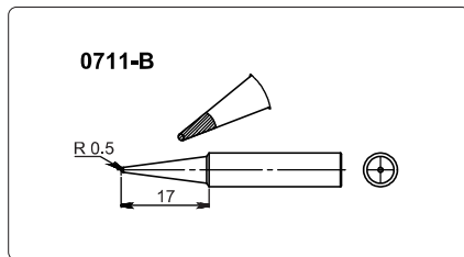
soldering tips (included)
